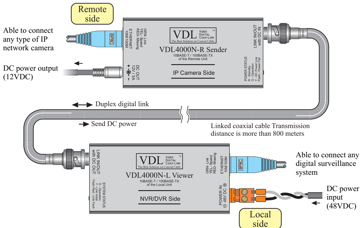
Fig.2 VDL4000N Connection Diagrams
